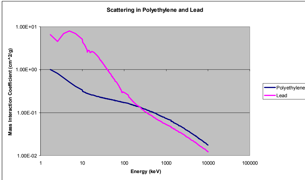
Figure 3.22 Mass Interaction Coefficient (coherent and incoherent scattering) for polyethylene and lead
