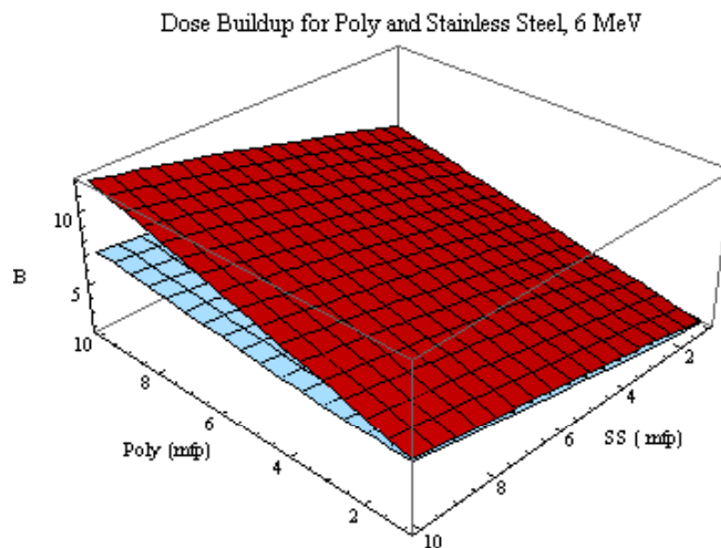
Figure 3.361 Dose Buildup Factors for 6 MeV photons incident on shields of polyethylene and stainless steel of varying thicknesses. The blue surface is stainless steel followed by polyethylene and the red is polyethylene followed by stainless steel.
