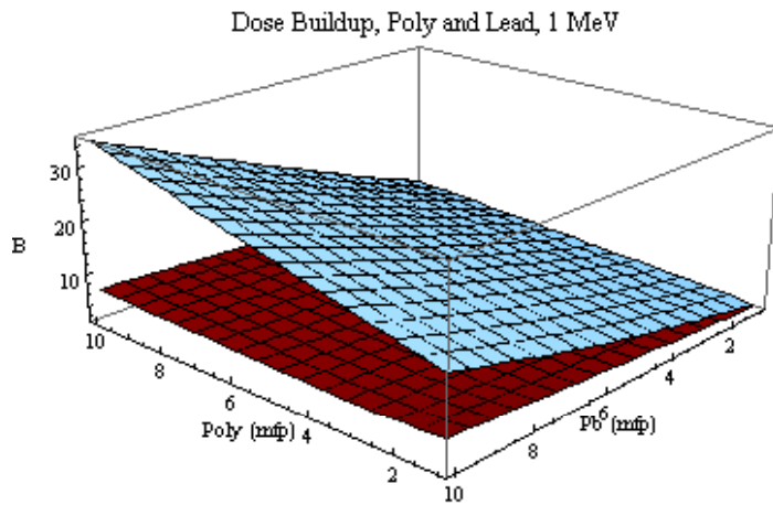
Figure 3.241 Dose Buildup Factors for 1 MeV photons incident on shields of polyethylene and lead of varying thicknesses The blue surface lead followed by polyethylene and the red is polyethylene followed by lead.
