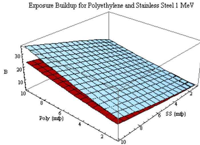
Figure 3.342 Exposure Buildup Factors for 1 MeV photons incident of shields of polyethylene and stainless steel of varying thicknesses. The blue surface is stainless steel followed by polyethylene and the red is polyethylene followed by stainless steel.
