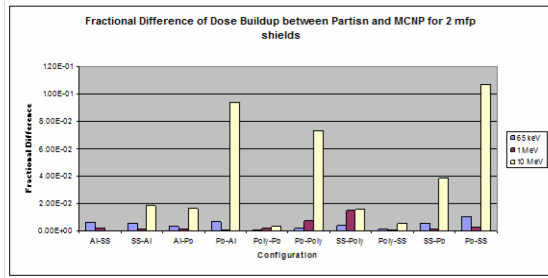
Figure 4.11 Absolute fractional differences between PARTISN flux calculations and MCNP5 Flux Calculations.
